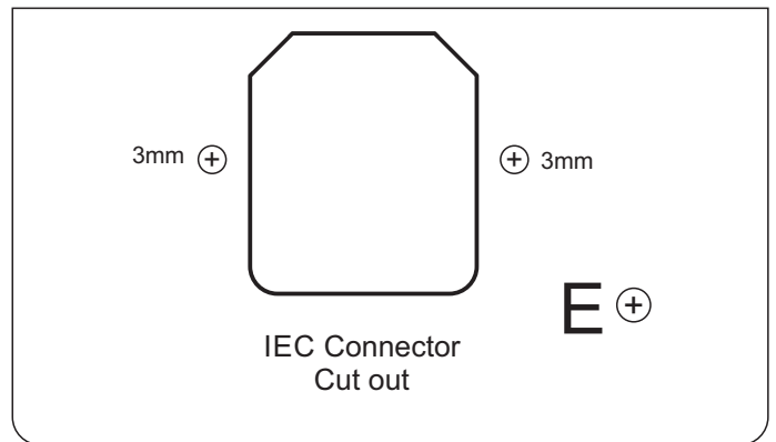
box end
