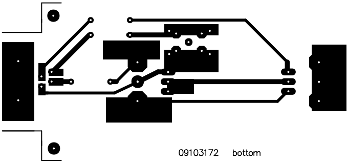
Tl_Hbridge2PWM
