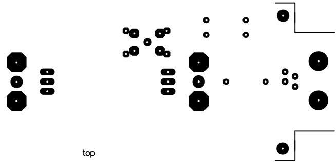
Tl_Hbridge2PWM
