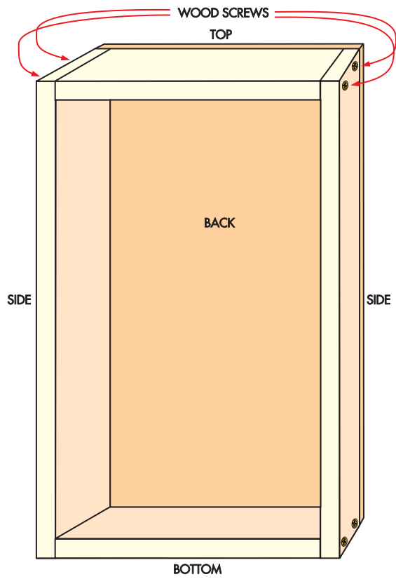
WS1000 SUBWOOFER BOX ASSEMBLY
