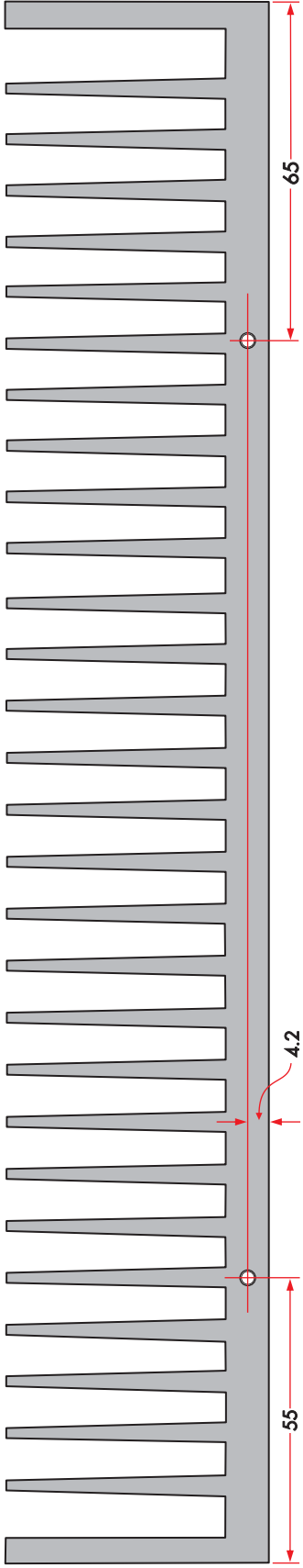
TOP VIEW (BOTTOM IS IDENTICAL)
